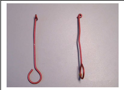
Pig Tail Wood frame brick veneer brick tie
